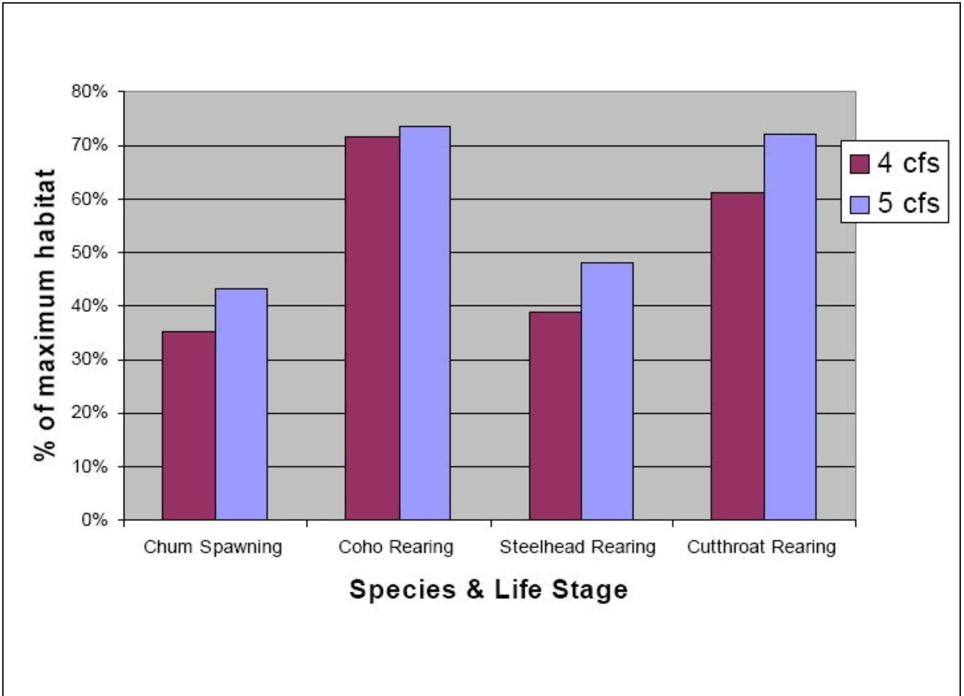
Figure 3.1-13. Barker Creek Habitat Available at Low Flows
