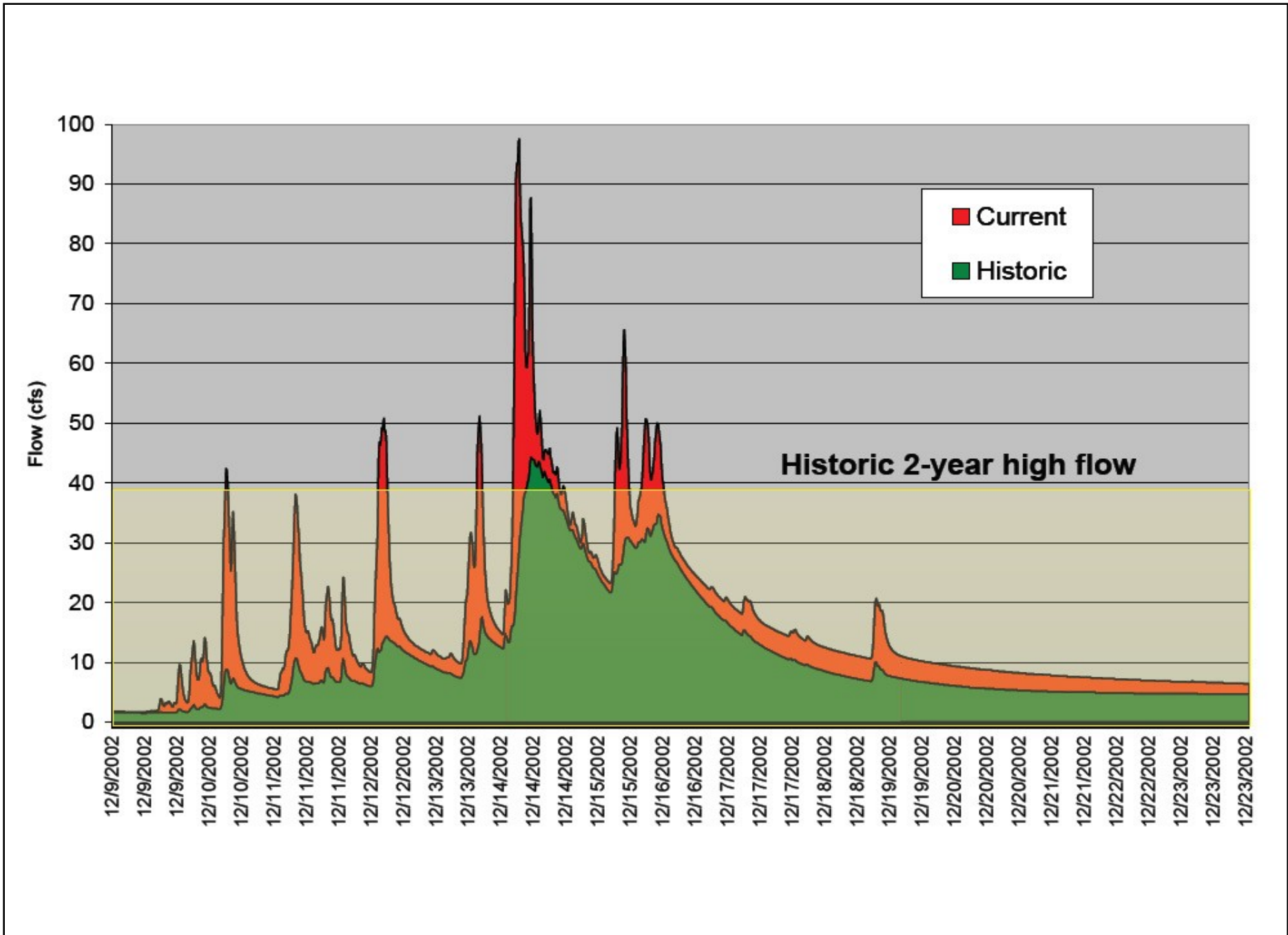
Figure 3.1-14. Barker Creek Hydrograph: Historic v. Current Flows for a 2-Week Rainy Period
