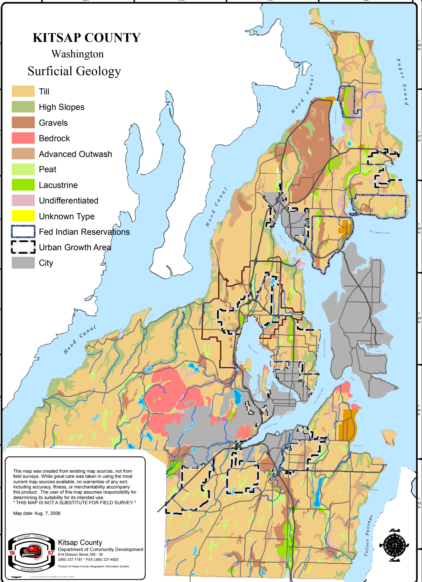
Figure 3.1-2 Surficial Geology
