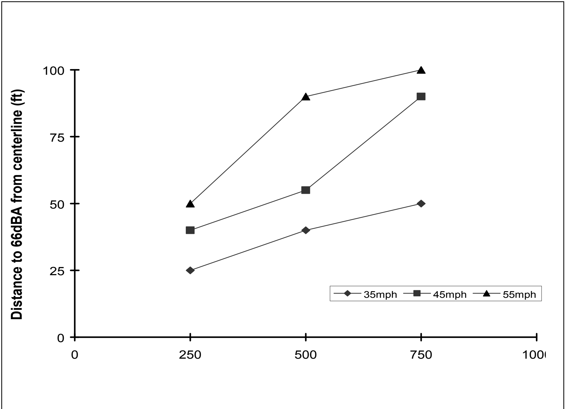
Figure 3.2-20. Estimated Noise Levels on a 2-Lane Roadway
