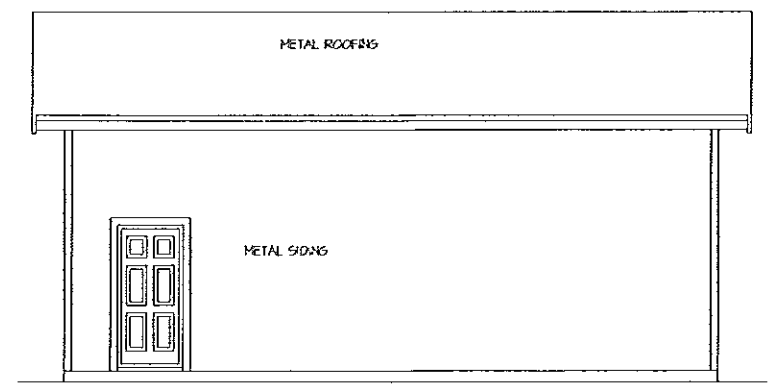
RIGHT ELEVATION 1/4" = 1'-0"
