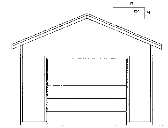
FRONT ELEVATION 1/4" = 1'-0"
