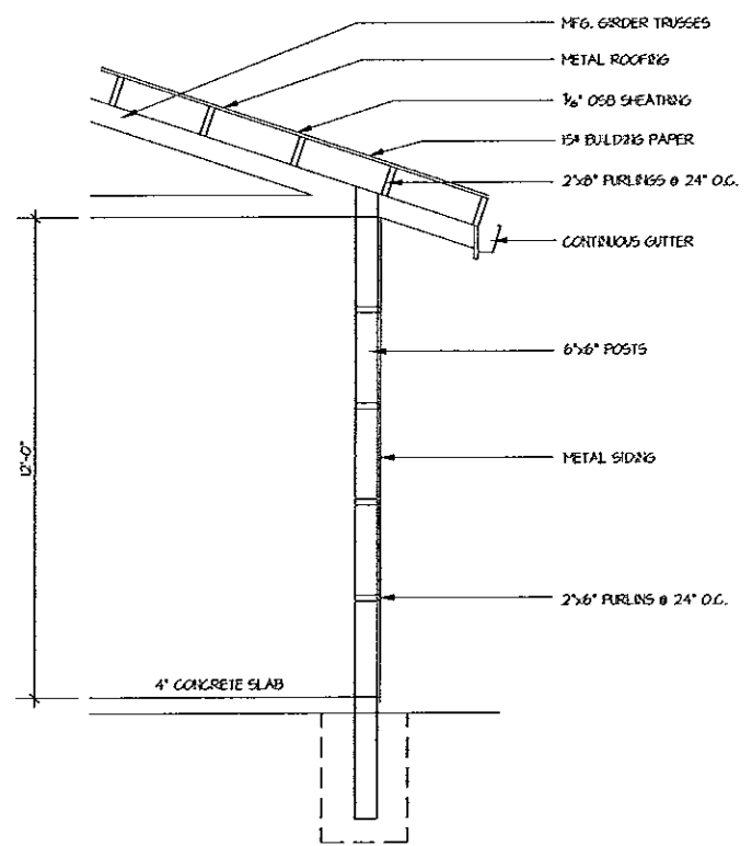
CROSSSECTION 1/2" = 1'-0"
