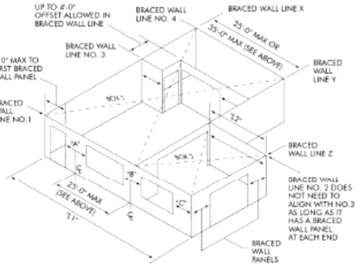
IBC Figure 2308.9.3, Basic Components of the Lateral Bracing System
