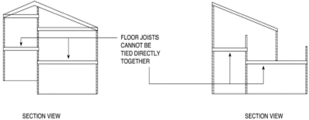
FIGURE 2308.12.6(6) PORTIONS OF FLOOR LEVEL OFFSET VERTICALLY
