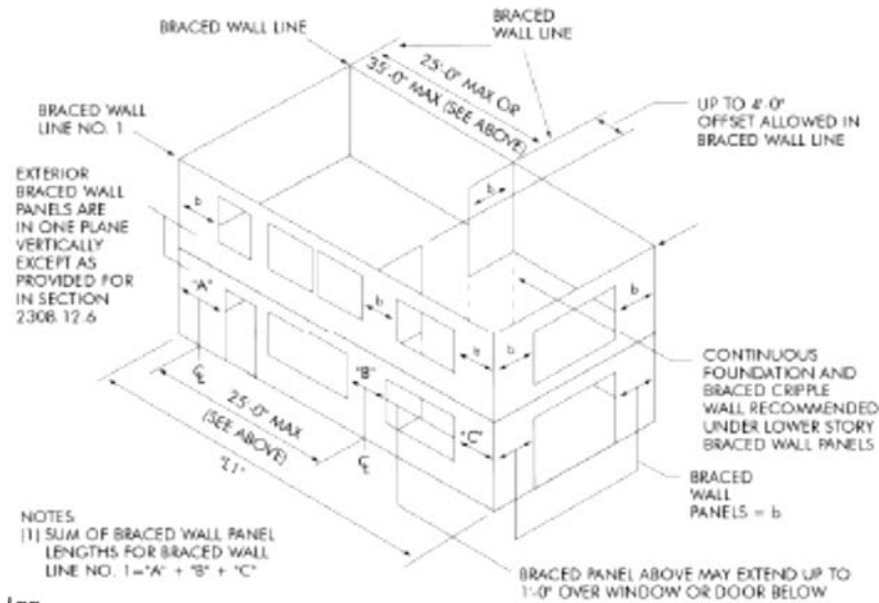
IBC Figure 2308.9.3, Basic Components of the Lateral Bracing System
